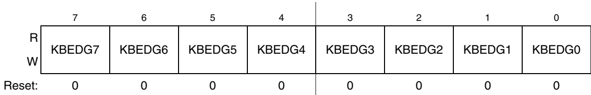
Figure 9-5. KBI Edge Select Register
