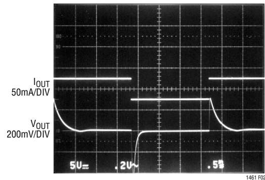
Figure 2. 50\text{mA} Load Step with C_L = 2\mu\text{F}
