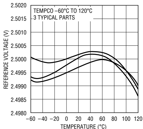
2.5V Reference Voltage vs Temperature
