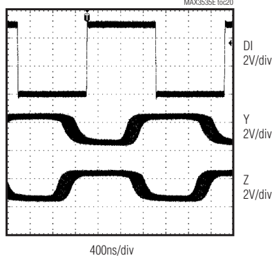
DRIVER PROPAGATION DELAY ( SLO = \text{LOW} )
