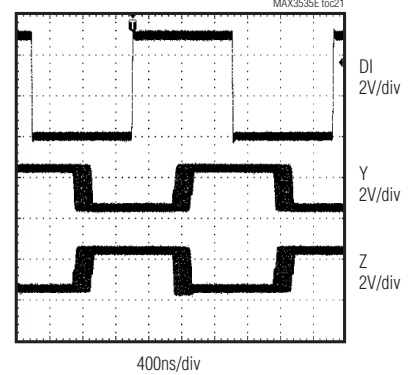
DRIVER PROPAGATION DELAY ( SLO = \text{HIGH} )
