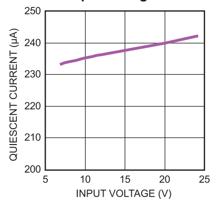
Supply Current (Quiescent) vs. Input Voltage
