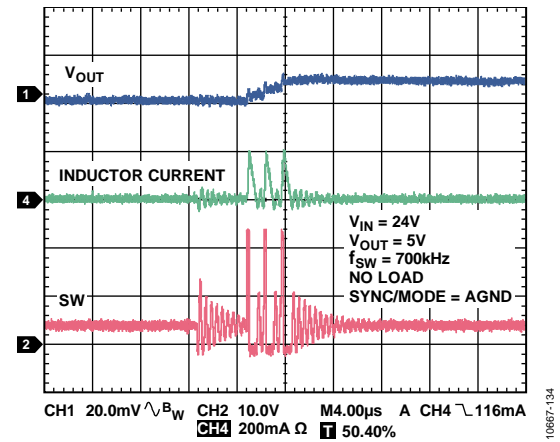
Figure 33. Pulse Skip Mode, V_{IN} = 24V , V_{OUT} = 5V , f_{SW} = 700kHz , No Load, SYNC/MODE = AGND
