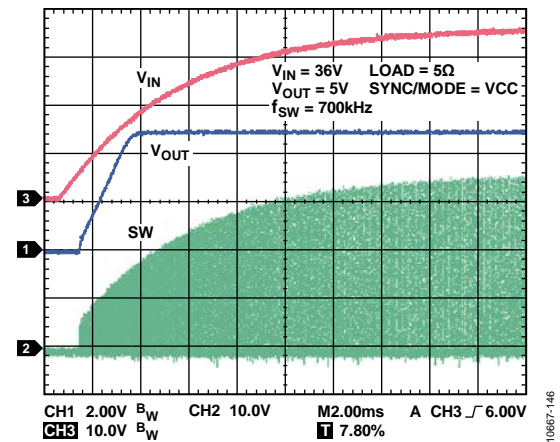
Figure 45. Startup with V_{IN} PWM Mode, V_{IN} = 36V , V_{OUT} = 5V , f_{SW} = 700kHz , Load = 5Ω, SYNC/MODE = VCC
