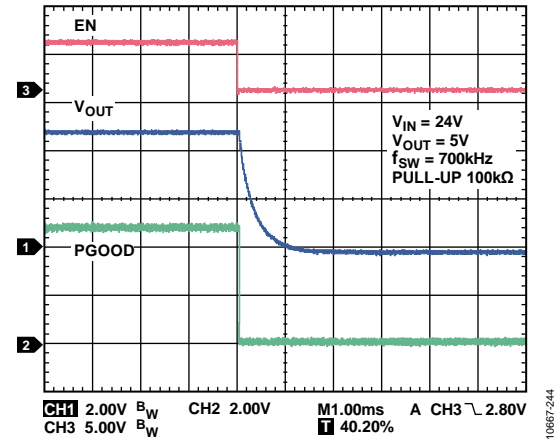
Figure 43. Power-Good Shutdown, V_{IN} = 24V , V_{OUT} = 5V , f_{SW} = 700kHz
