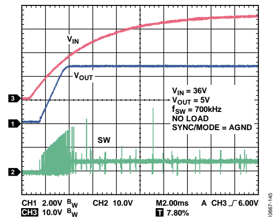
Figure 44. Startup with V_{IN} Pulse Skip Mode, V_{IN} = 36V , V_{OUT} = 5V , f_{SW} = 700kHz , No Load, SYNC/MODE = AGND
