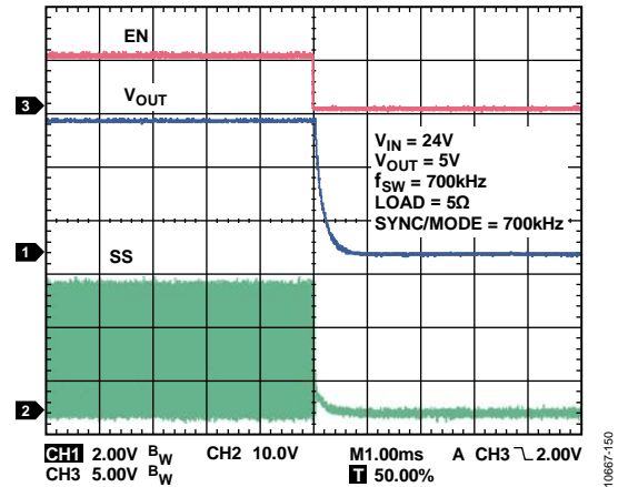
Figure 49. Shutdown with Precision Enable, V_{IN} = 24V , V_{OUT} = 5V , f_{SW} = 700kHz , Load = 5Ω, SYNC/MODE = 700kHz
