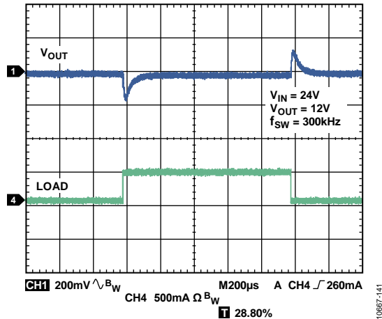
Figure 40. Load Transient Response, V_{IN} = 24V , V_{OUT} = 12V , f_{SW} = 300kHz , SYNC/MODE = Clock, Load Step = 500mA
