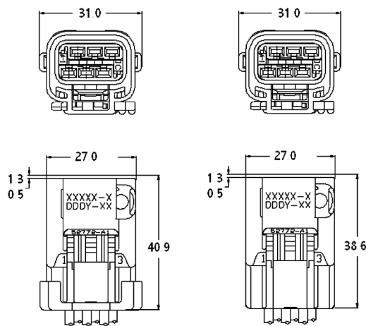
Sealed Assembly
