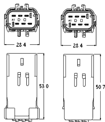
Sealed Assembly
