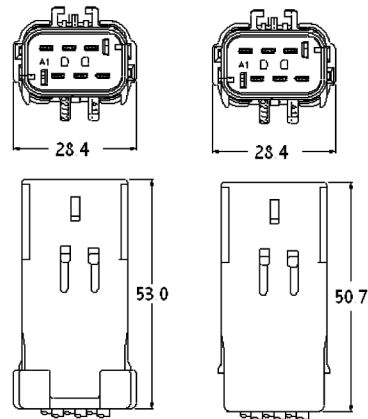
Sealed Assembly
