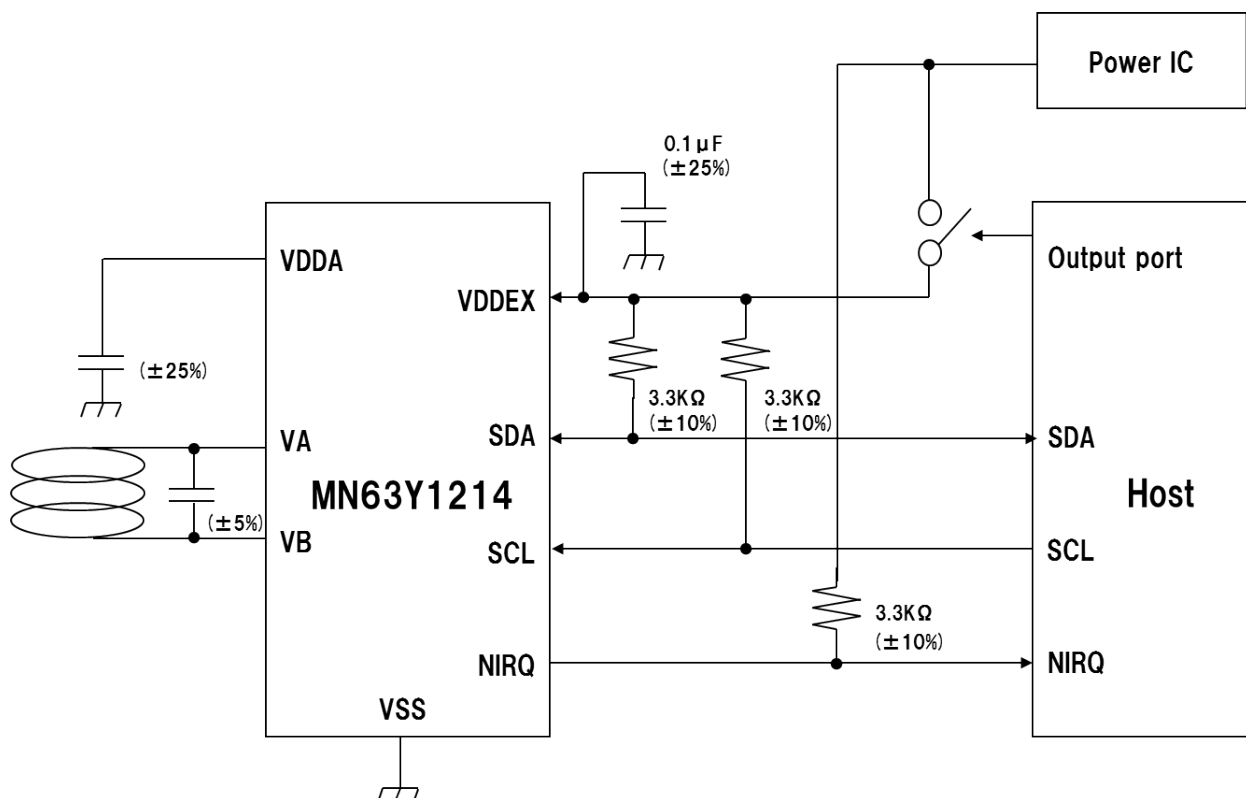
Figure 2-3 Connection Example
