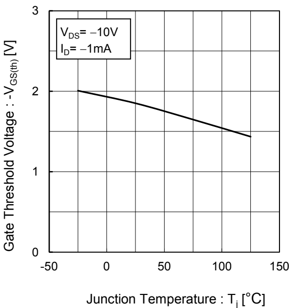
Fig.11 Gate Threshold Voltage vs. Junction Temperature
