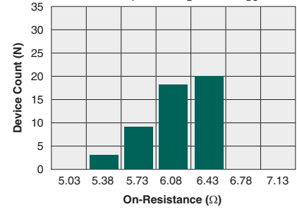
Typical On-Resistance Distribution (N=50, I_F=5mA, I_L=200mA_{DC} )
