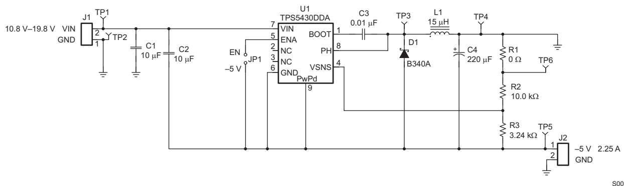
Figure 10. TPS5430EVM-342 Schematic
