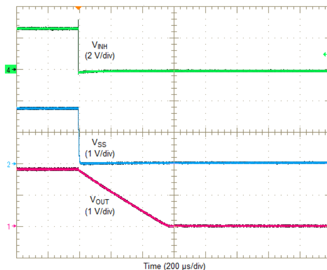
Figure 30. Inhibit Turn-Off
