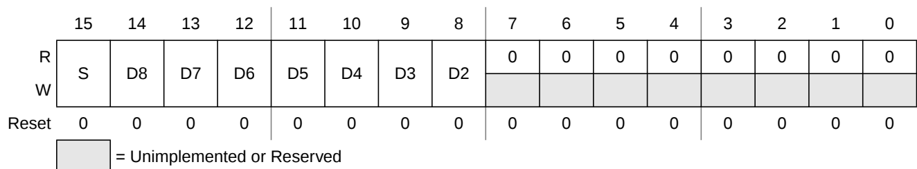
Figure 9-9. Motor Controller Duty Cycle Register x (MCDxCx) with FAST = 1
