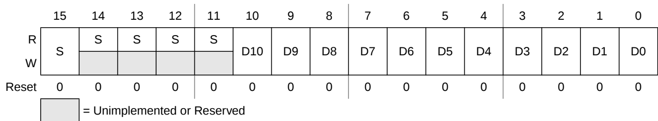
Figure 9-8. Motor Controller Duty Cycle Register x (MCDxCx) with FAST = 0
