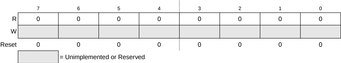
Figure 21-6. Reserved Register
