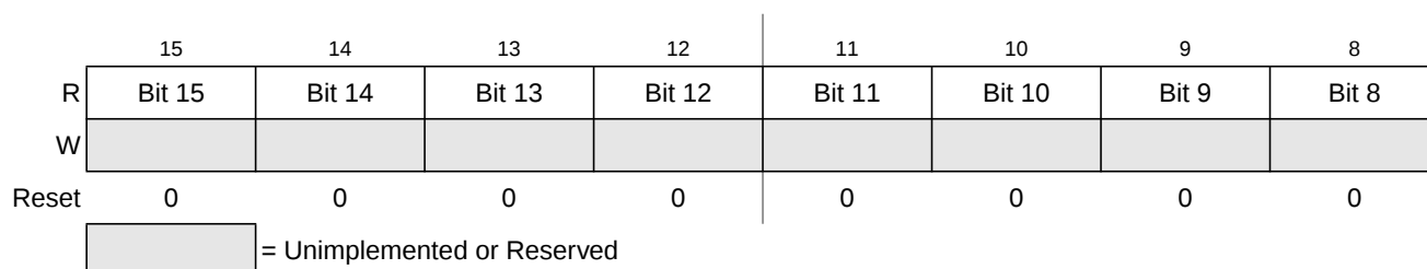
Figure 19-11. Debug Comparator C Register High (DBG CCH)
