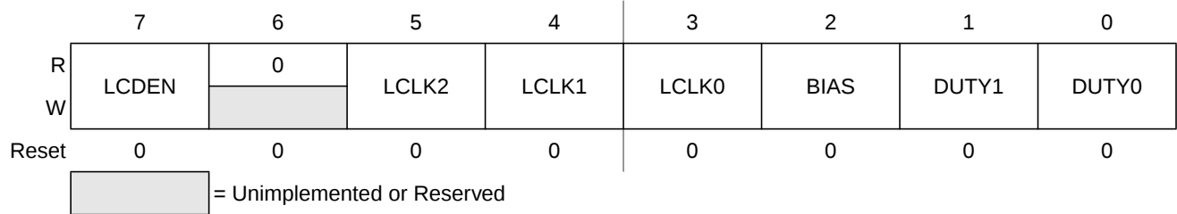
Figure 8-2. LCD Control Register 0 (LDCR0)
