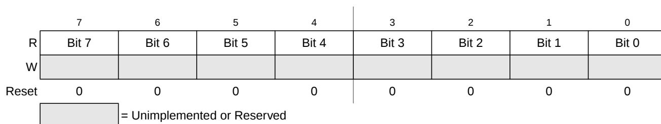
Figure 19-12. Debug Comparator C Register Low (DBG CCL)
