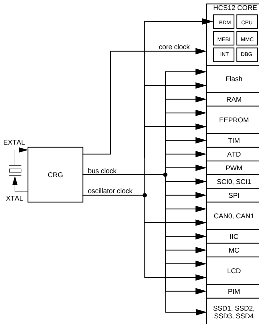
Figure 1-12. Clock Connections
