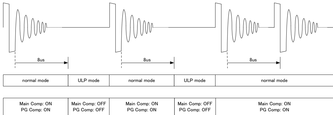
Figure 5. Transition between Normal Mode and ULP Mode
