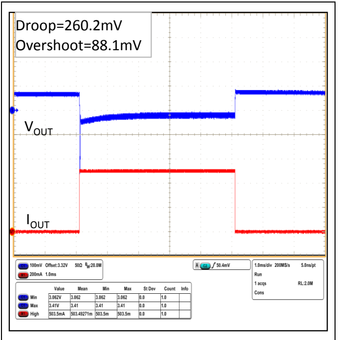
Figure 26. Load Transient Response ( V_{IN} =3.6V, V_{OUT} =3.3V, I_{OUT} =1uA \leftrightarrow 500mA, t_r = t_f =1 \mu s)
