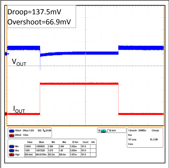
Figure 24. Load Transient Response ( V_{IN} =3.6V, V_{OUT} =1.8V, I_{OUT} =1uA \leftrightarrow 500mA, t_r = t_f =1 \mu s)
