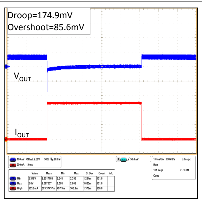
Figure 25. Load Transient Response ( V_{IN} =3.6V, V_{OUT} =2.5V, I_{OUT} =1uA \leftrightarrow 500mA, t_r = t_f =1 \mu s)
