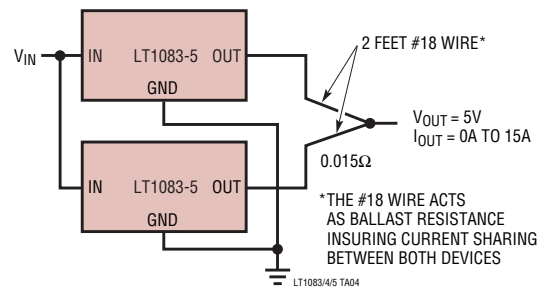
Paralleling Regulators
