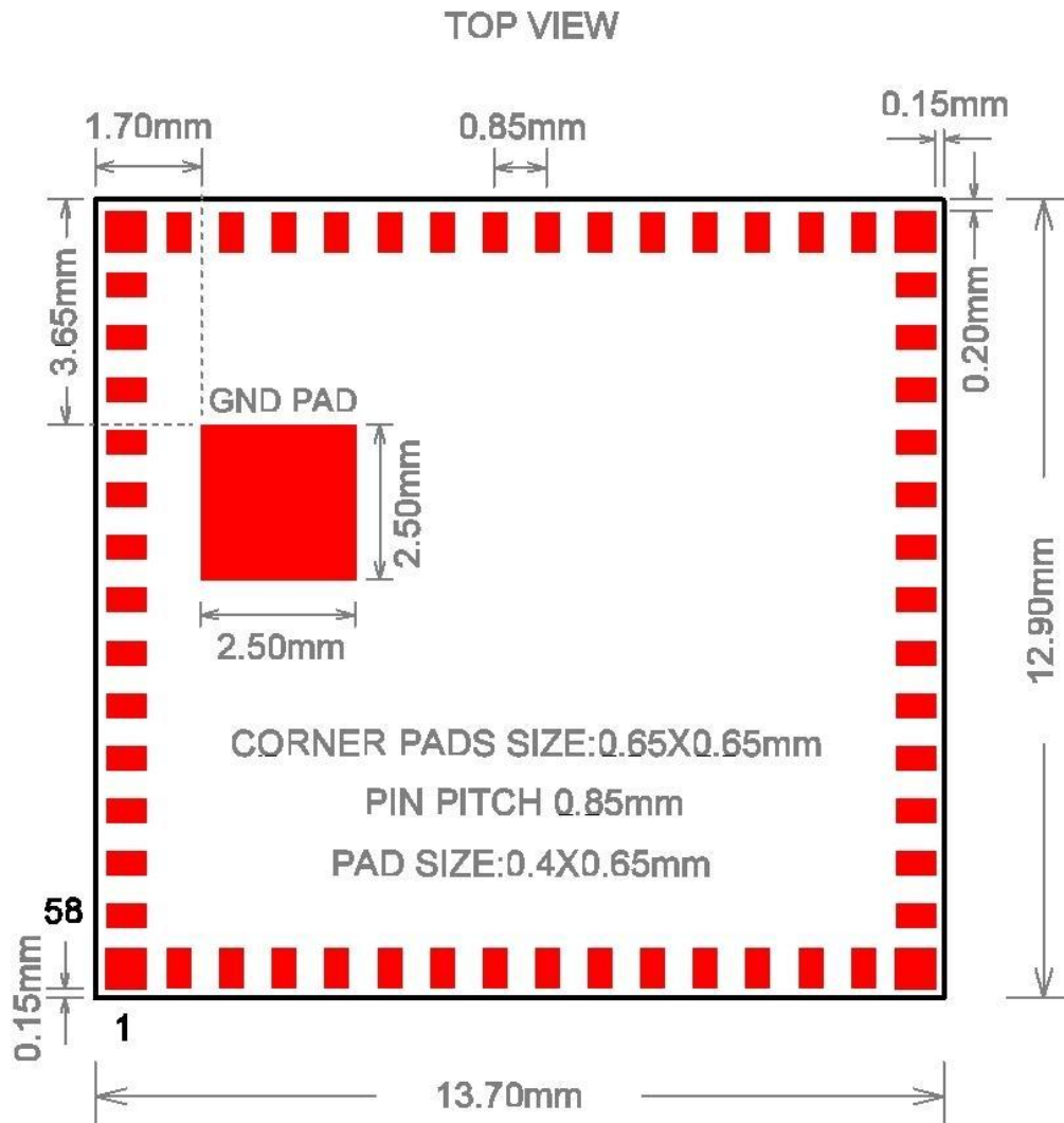
Figure 3: Package Dimensions
