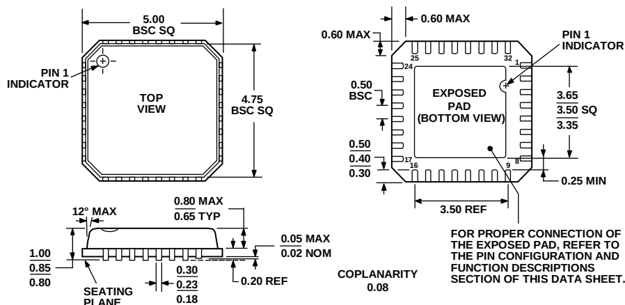
Figure 66. 32-Lead Lead Frame Chip Scale Package [LFCSP_VQ] 5 mm × 5 mm Body, Very Thin Quad (CP-32-4)
