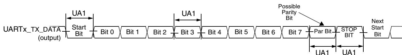
Figure 49. UART RS-232 Serial Mode Transmit Timing Diagram
