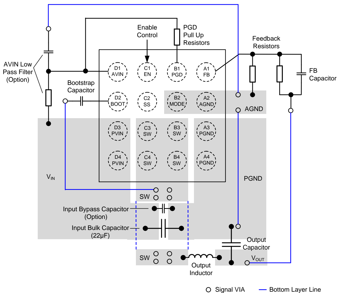
Figure 76. Example of PCB Layout (TOP VIEW)
