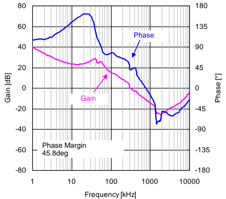
Figure 69. Closed Loop Response I_{OUT} = 1A ( V_{IN} = 5V , V_{OUT} = 3.3V , L = 1.5\mu H , C_{OUT} = 22\mu F )
