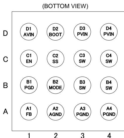
Figure 2. Pin Configuration
