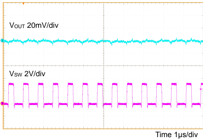
Figure 30. Switching Waveform (V_{PVIN} = V_{AVIN} = 3.3V, V_{OUT} = 0.9V, V_{MODE} = 0V, I_{OUT} = 3A)
