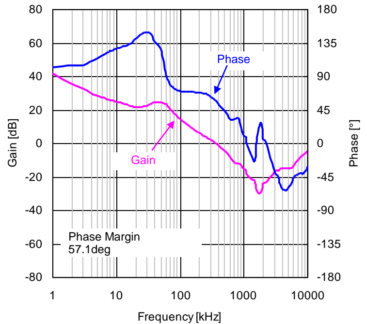
Figure 59. Closed Loop Response I_{OUT} = 1A ( V_{IN} = 5V , V_{OUT} = 1.2V , L = 1.0\mu H , C_{OUT} = 22\mu F )
