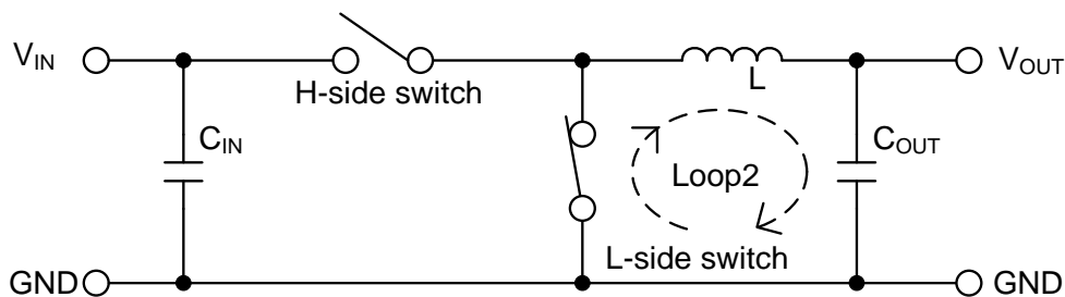
Figure 75-b. Current path when H-side switch = OFF, L-side switch = ON
