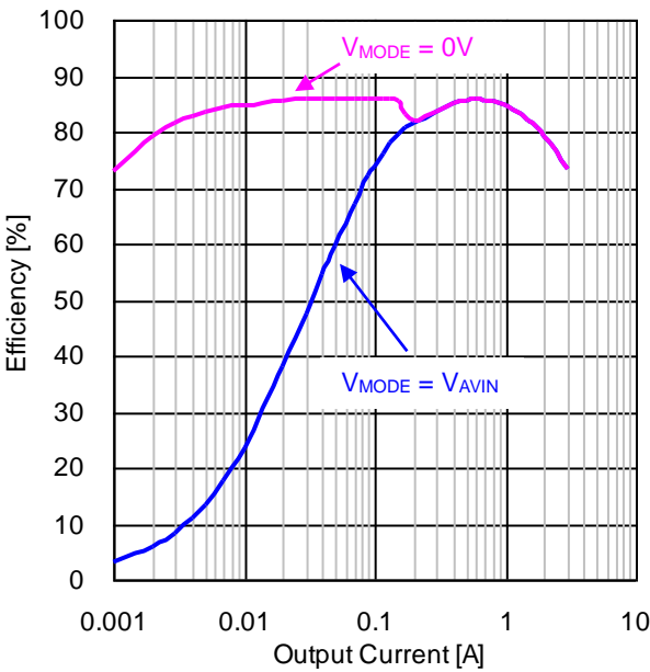
Figure 38. Efficiency vs Output Current ( V_{PVIN}=V_{AVIN}=3.3V , V_{OUT}=0.9V , L=1.0\mu H )
