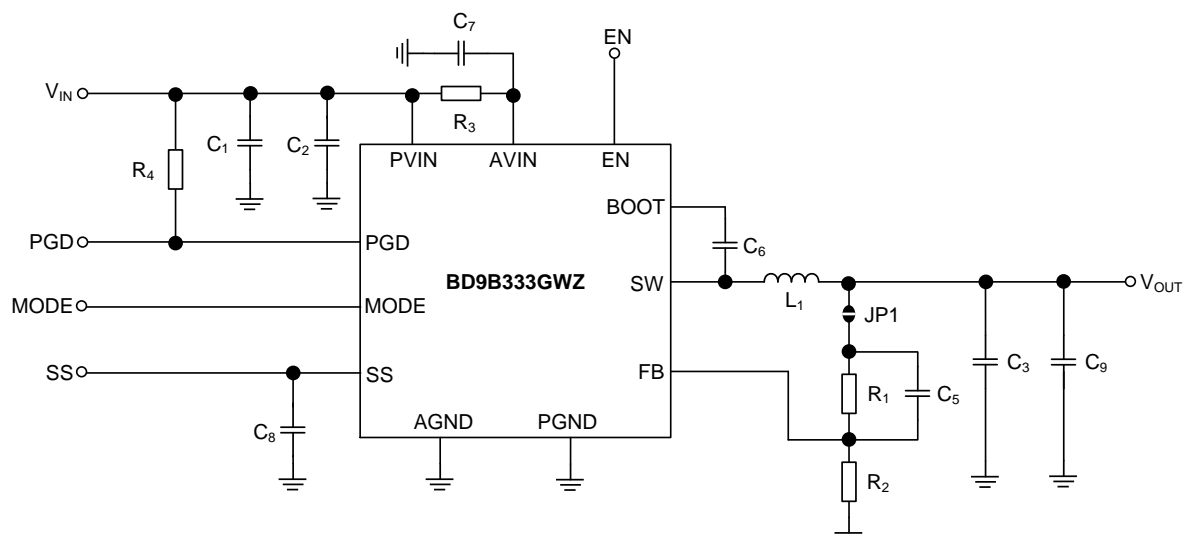
Figure 52. Application Circuit
