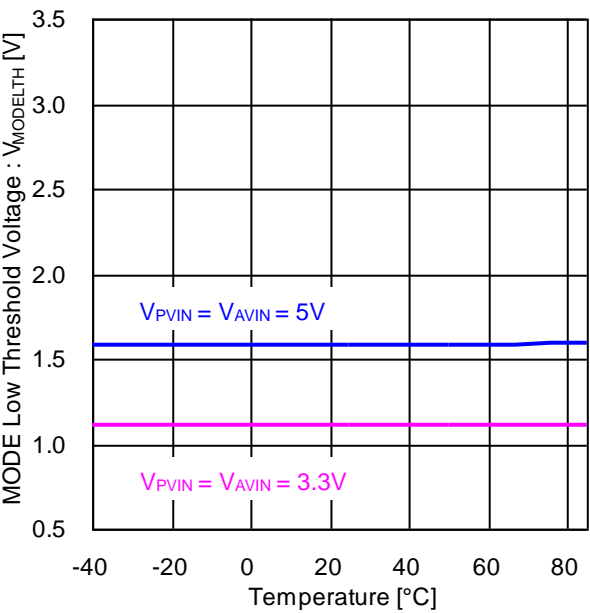
Figure 15. MODE Low Threshold Voltage vs Temperature
