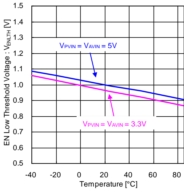
Figure 8. EN Low Threshold Voltage vs Temperature ( V_{EN} Sweep Down)
