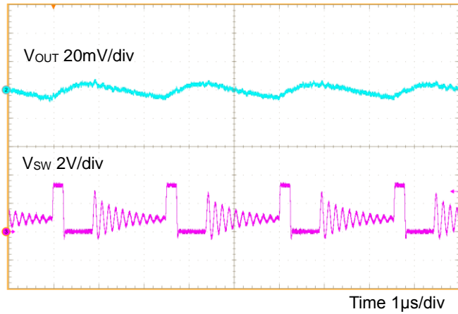
Figure 28. Switching Waveform (V_{PVIN} = V_{AVIN} = 3.3V, V_{OUT} = 0.9V, V_{MODE} = 0V, I_{OUT} = 0.1A)
