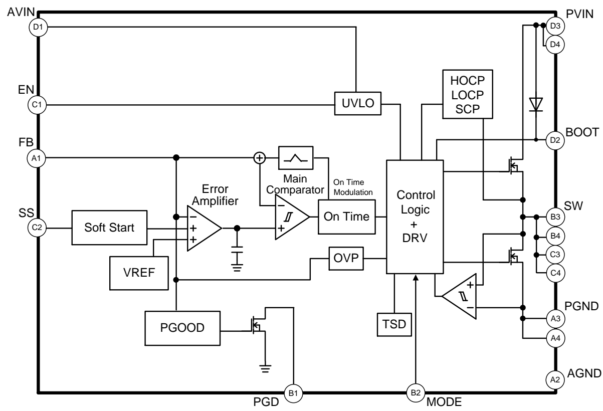
Figure 3. Block Diagram
