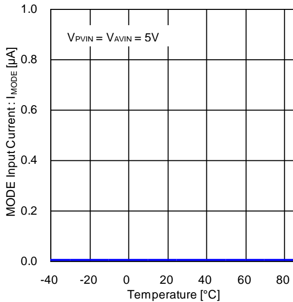
Figure 16. MODE Input Current vs Temperature ( V_{MODE} = 5V )
