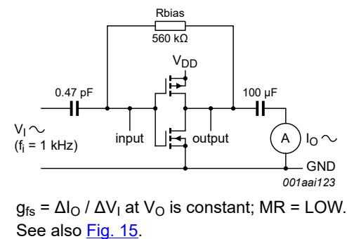
Fig. 14. Test set-up for measuring forward transconductance
