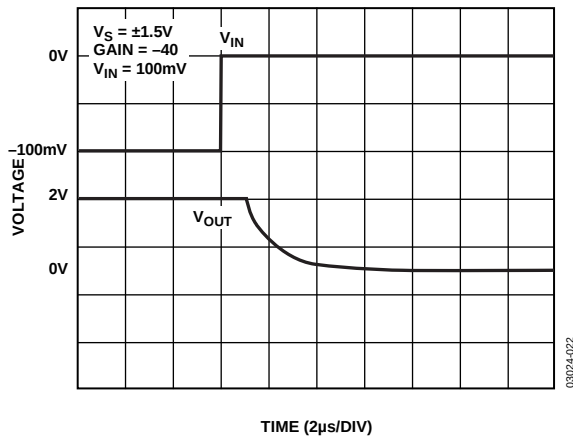
Figure 22. Saturation Recovery
