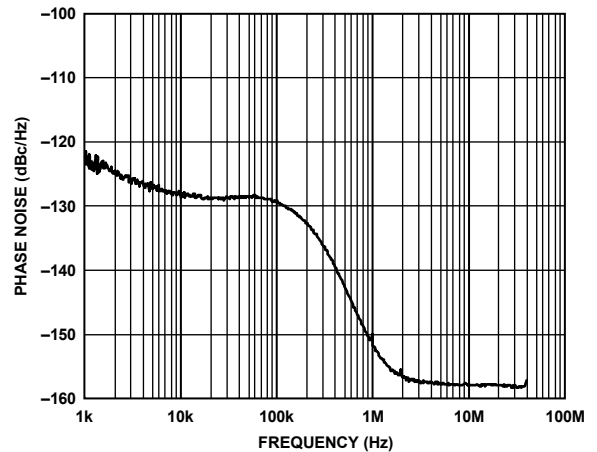
Figure 9. Phase Noise, PLL1, OUT0 LVPECL, 100 MHz, Integer-N Mode ( f_{XTAL} = 25 MHz, N_a = 100 , V_0 = 5 , D_0 = 5 )
