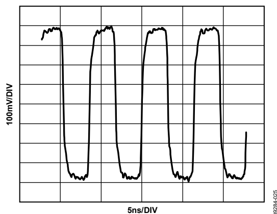
Figure 21. Typical LVDS Differential Output Trace, 156.25 MHz
