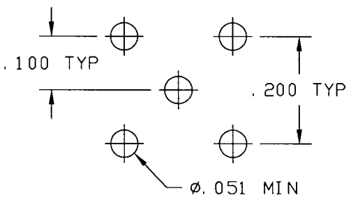
MOUNTING DIMENSIONS
