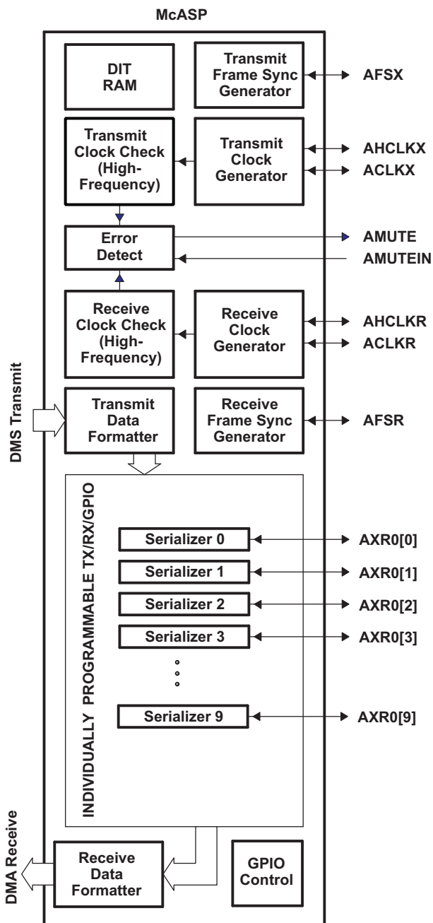
Figure 6-48. McASP Configuration
