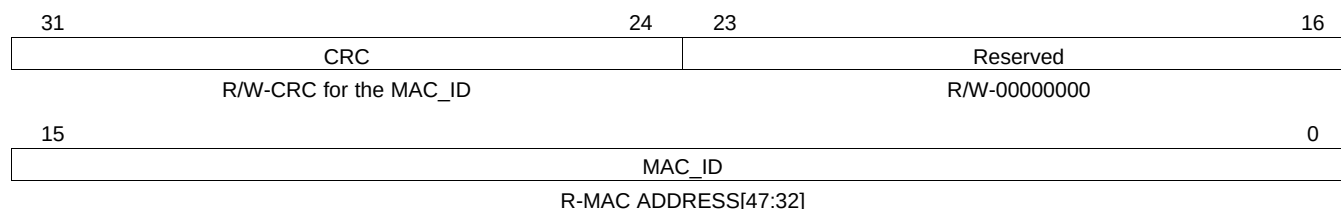
Figure 3-10. MAC_ADDR_RW1 Register
