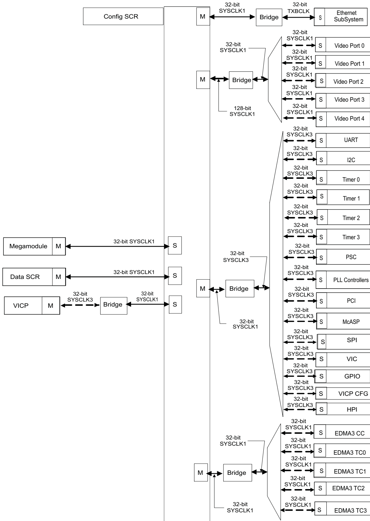
Figure 4-2. Configuration SCR
