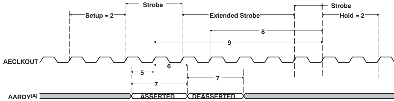
Figure 6-23. AARDY Timing
