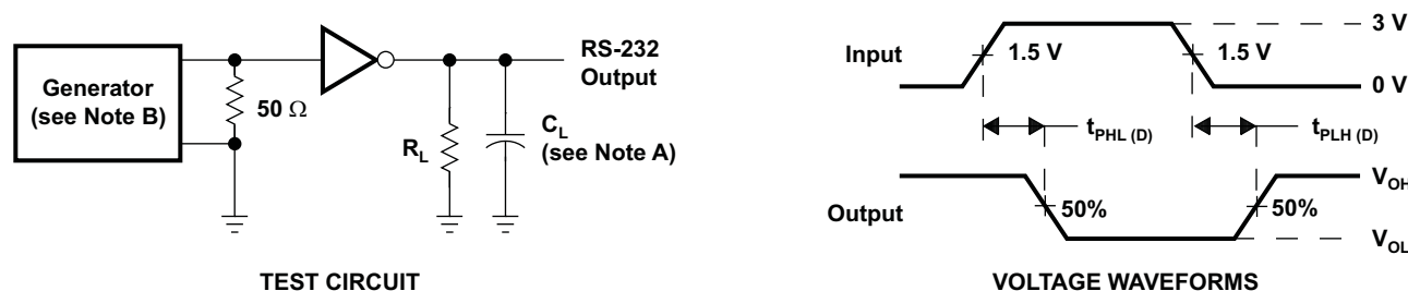
Figure 2. Driver Slew Rate
