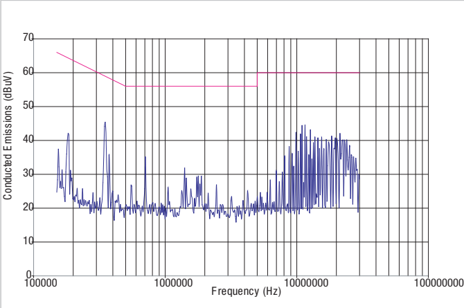
NPH10S4803
