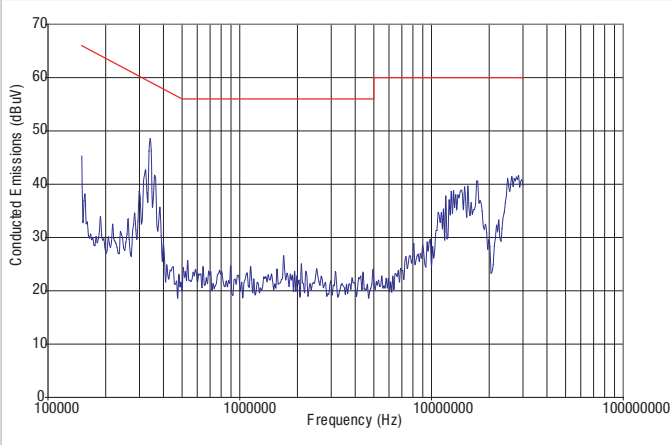
NPH10S2412
