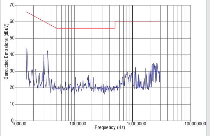
NPH10S2405
