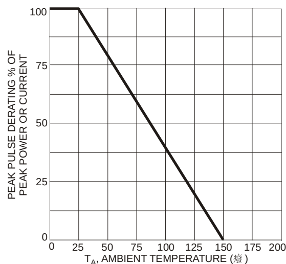
Figure 2 Pulse Derating C(°C)
