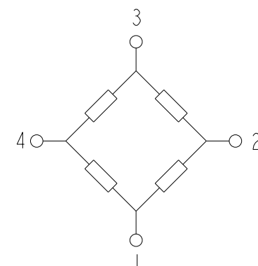
EQUIVALENT CIRCUIT
