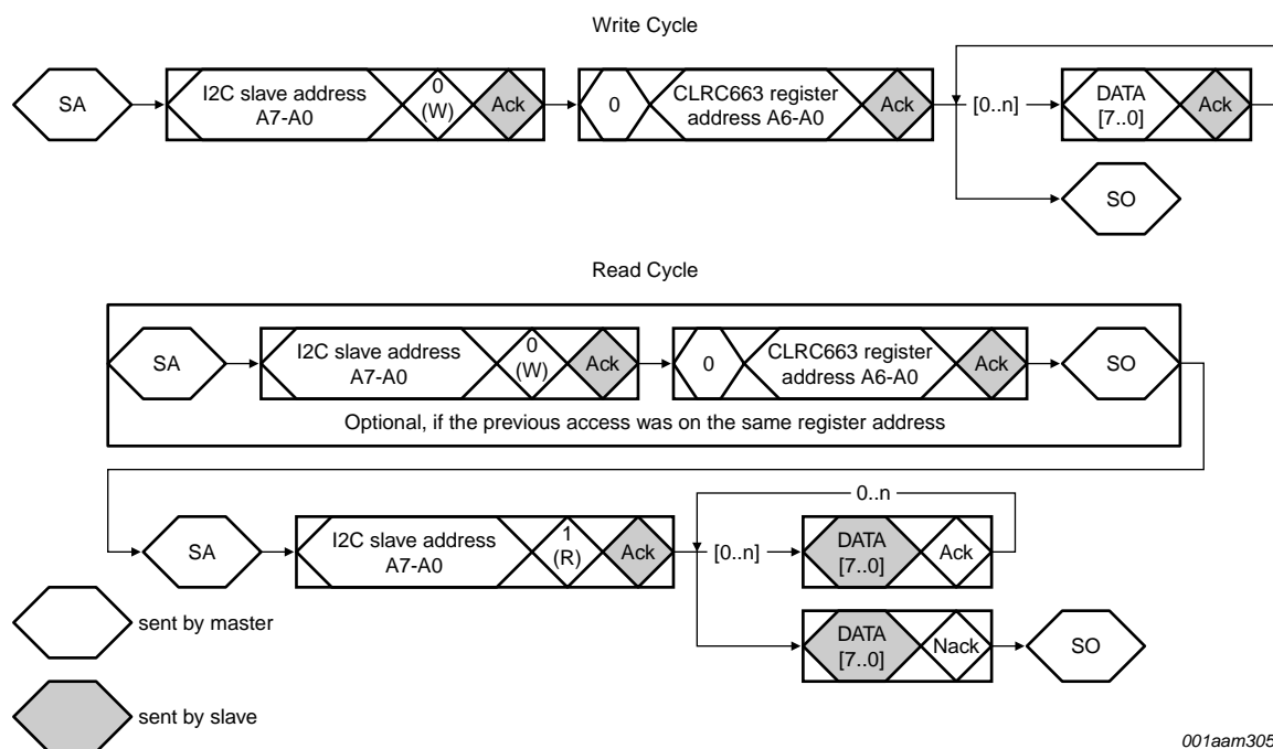
Fig 17. Register read and write access
