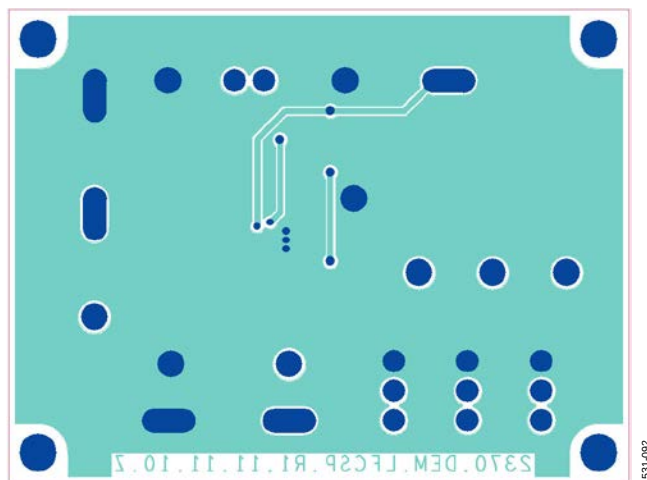
Figure 92. PCB Layout, Bottom
