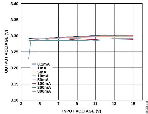
Figure 11. Line Regulation, V_{OUT} = 3.3\text{ V} , Different Loads
