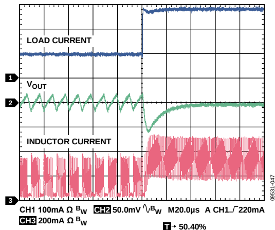
Figure 47. Load Transient, V_{OUT} = 1.2\text{ V} , 100 mA to 300 mA, Load Current Rise Time = 200 ns, V_{IN} = 5\text{ V}
