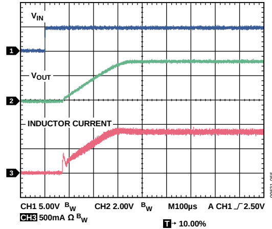
Figure 55. Startup, V_{OUT} = 3.3V , 800 mA
