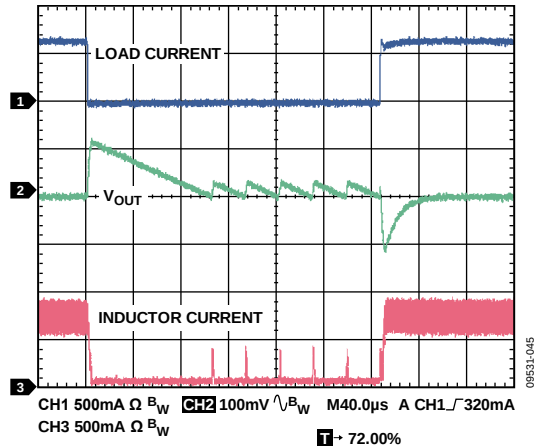
Figure 45. Load Transient, V_{OUT} = 1.2\text{ V} , 10 mA to 800 mA, Load Current Rise Time = 200 ns, V_{IN} = 5\text{ V}
