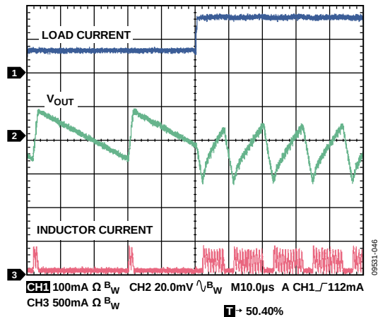
Figure 46. Load Transient, V_{OUT} = 1.2\text{ V} , 10 mA to 110 mA, Load Current Rise Time = 200 ns, V_{IN} = 5\text{ V}
