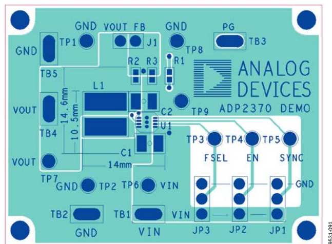
Figure 91. PCB Layout, Top
