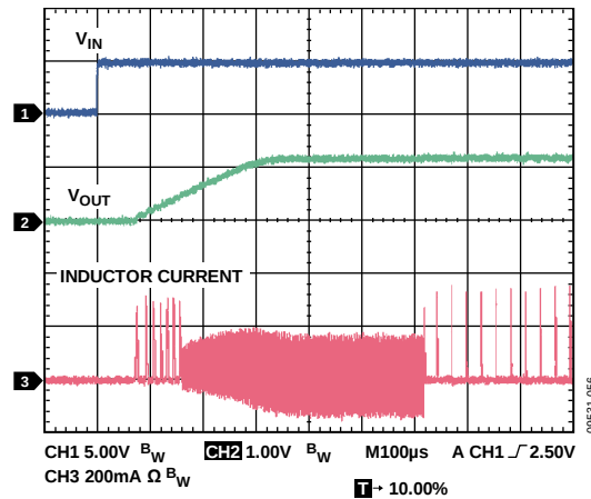
Figure 56. Startup, V_{OUT} = 1.2V , 10 mA, V_{IN} = 5V
