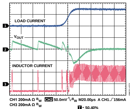
Figure 72. PSM to PWM Transition Waveforms, V_{OUT} = 1.8 V, 10 mA Load to 300 mA Load
