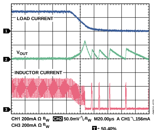
Figure 73. PWM to PSM Transition Waveforms, V_{OUT} = 1.8 V, 300 mA Load to 10 mA Load
