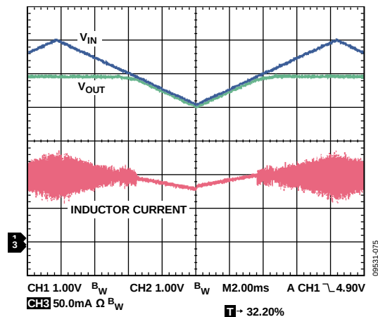
Figure 75. Transition into and out of Dropout in PWM Mode, V_{OUT} = 5\text{ V} , 100 mA Load
