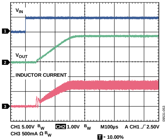
Figure 53. Startup, V_{OUT} = 1.8V , 800 mA
