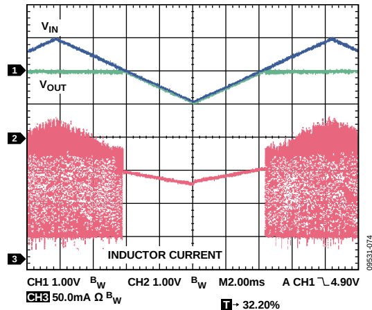
Figure 74. Transition into and out of Dropout in PSM Mode, V_{OUT} = 5\text{ V} , 100 mA Load
