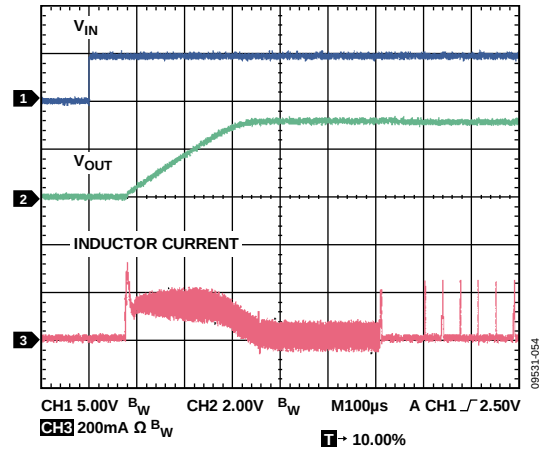
Figure 54. Startup, V_{OUT} = 3.3V , 10 mA
