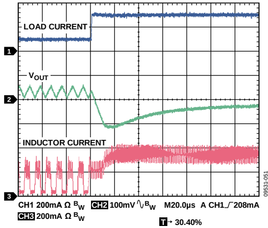
Figure 51. Load Transient, V_{OUT} = 5V , 100 mA to 300 mA, Load Current Rise Time = 200 ns, V_{IN} = 8V
