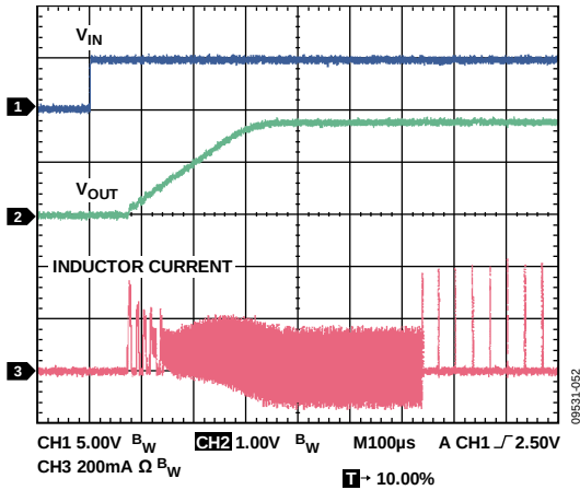
Figure 52. Startup, V_{OUT} = 1.8V , 10 mA
