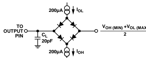
Figure 4. Load Circuit for SDO Timing Specifications
