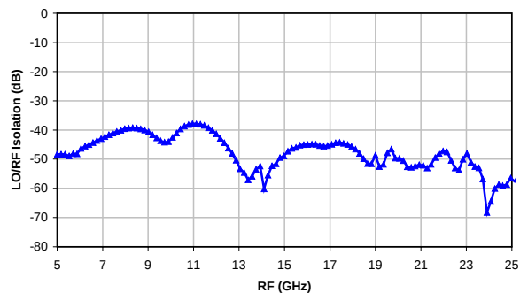
XR1011-QH: LO/RF Isolation (dB) vs. RF (GHz). 4 V @ 130mA, PLO = 5dBm
