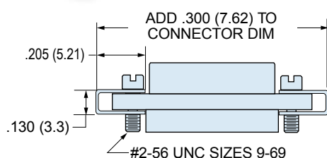
Figure 1 C Clip for Size 9 to Size 69 Pin Micro-D
