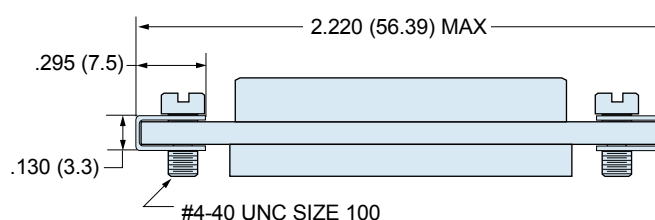
Figure 2 C Clip for Size 100 Micro-D
