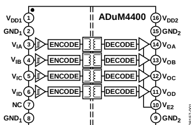
Figure 1. ADuM4400
