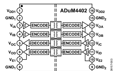
Figure 3. ADuM4402
