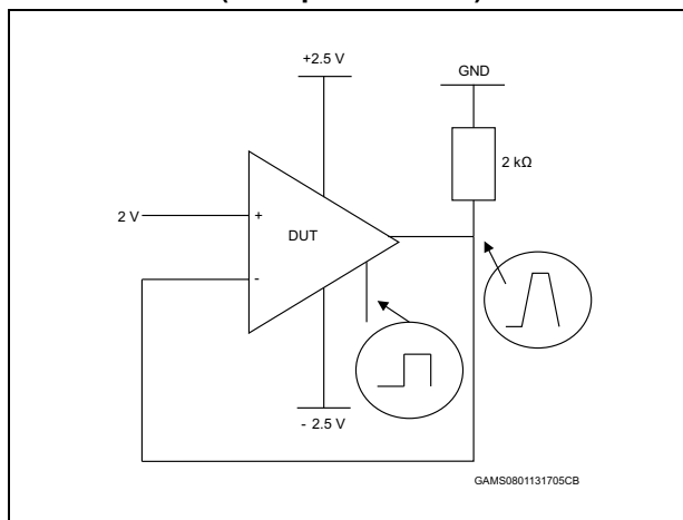
Figure 18. Test configuration for turn-on time (Vout pulled down)
