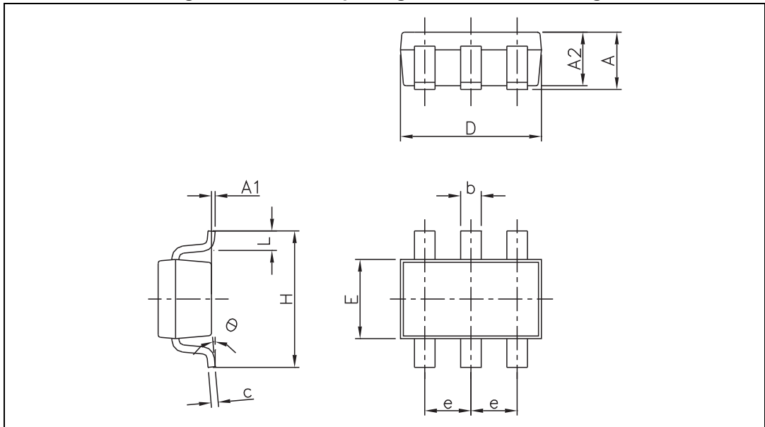
Figure 25. SOT23-6 package mechanical drawing
