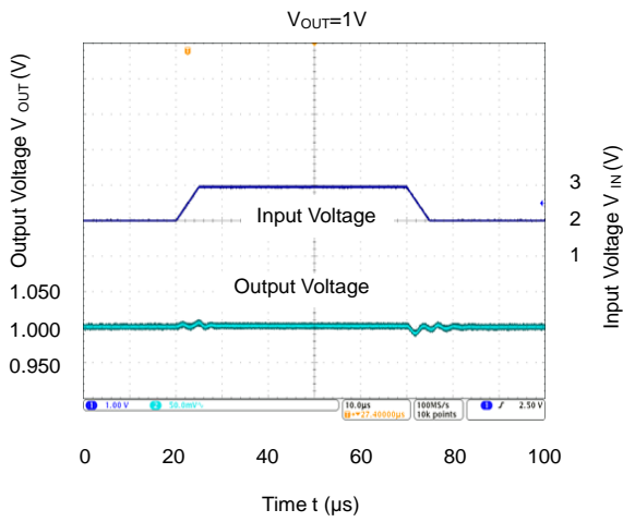
Line Transient Response Waveforms ( I_{OUT} = 30mA , t_R = t_F = 5\mu s , C_{IN} = \text{None} , C_{OUT} = 1\mu F , T_A = +25^\circ C )
