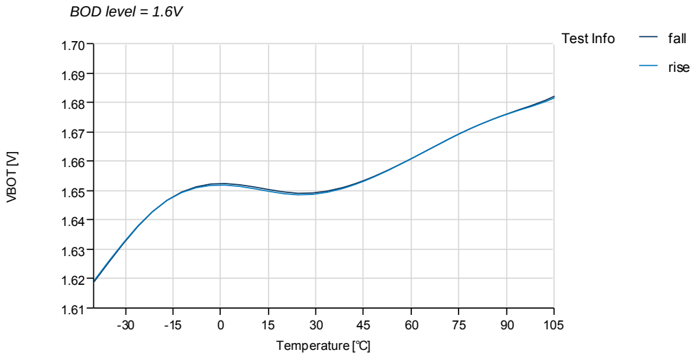
Figure 37-60.BOD thresholds vs. temperature.
