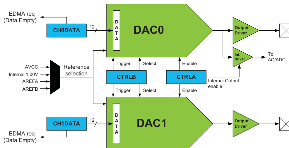
Figure 29-1. DAC overview.
