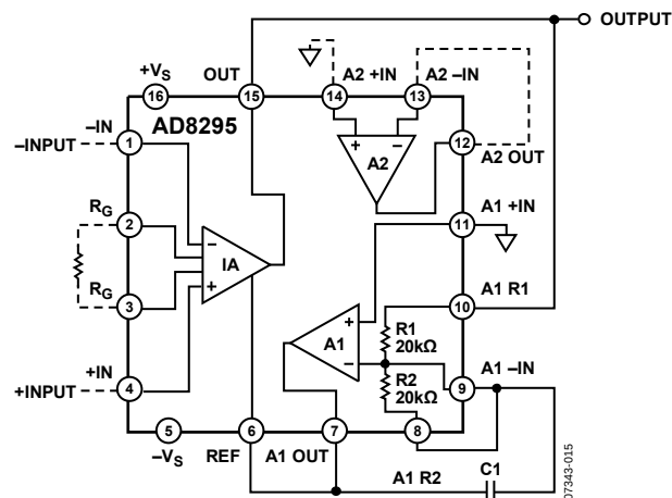
Figure 70. AC-Coupled Connection
