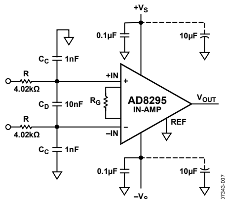
Figure 63. RFI Suppression
