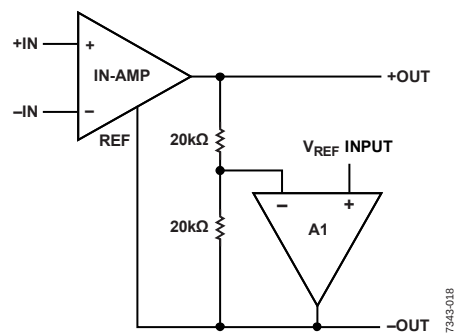
Figure 64. Differential Output Configuration Using an Op Amp
