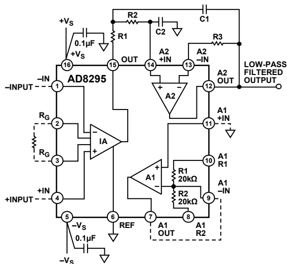
Figure 69. Two-Pole Sallen-Key Filter
