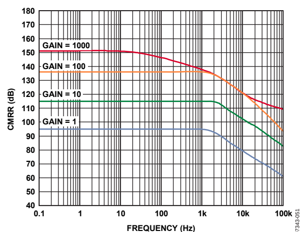
Figure 18. CMRR vs. Frequency, RTI, G = 1 to 1000
