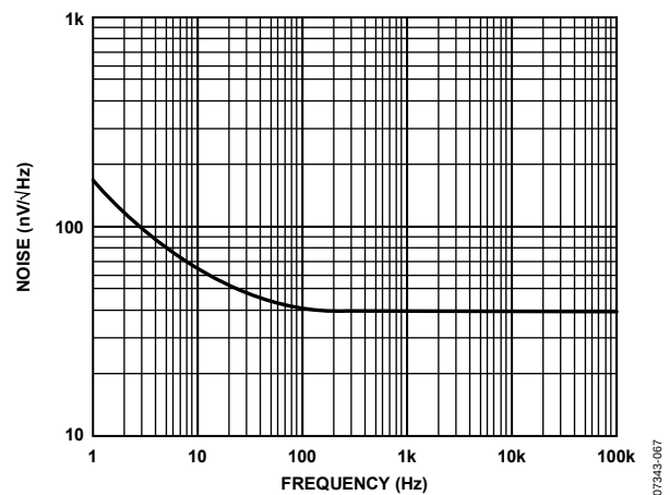
Figure 47. Voltage Noise Density vs. Frequency
