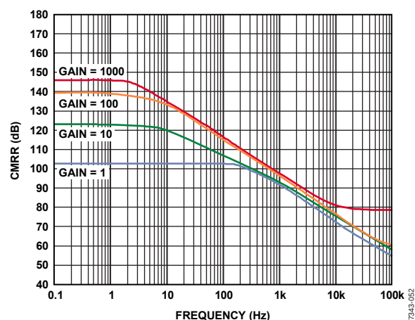
Figure 19. CMRR vs. Frequency, RTI, 1 kΩ Source Imbalance, G = 1 to 1000
