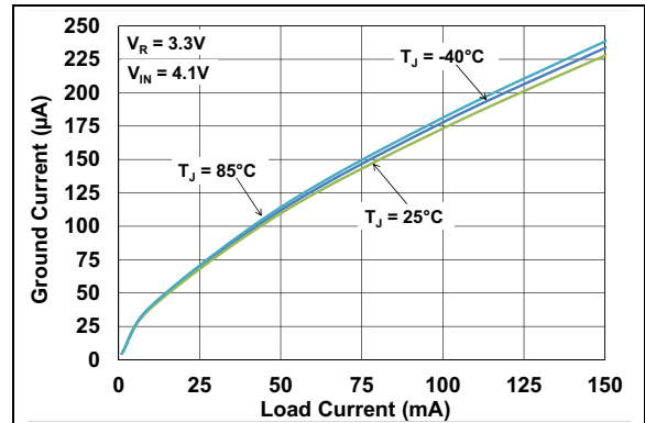
FIGURE 2-54: Ground Current vs. Load Current ( V_R = 3.3\text{V} ).
