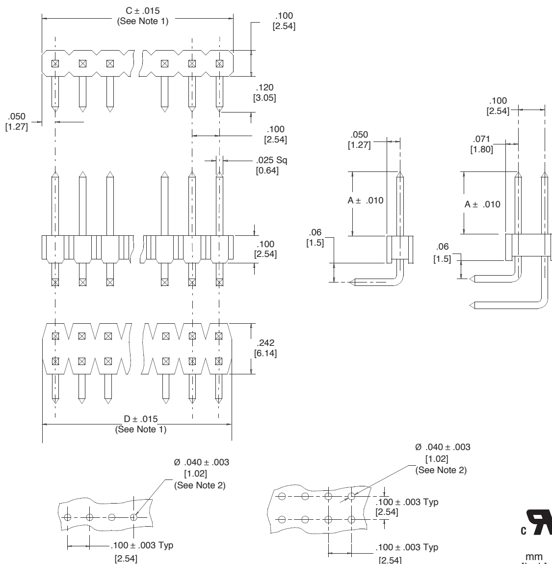
Recommended Mounting Hole Pattern
