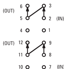
Bottom View for 4P-6, 4P-7, 4P-8
