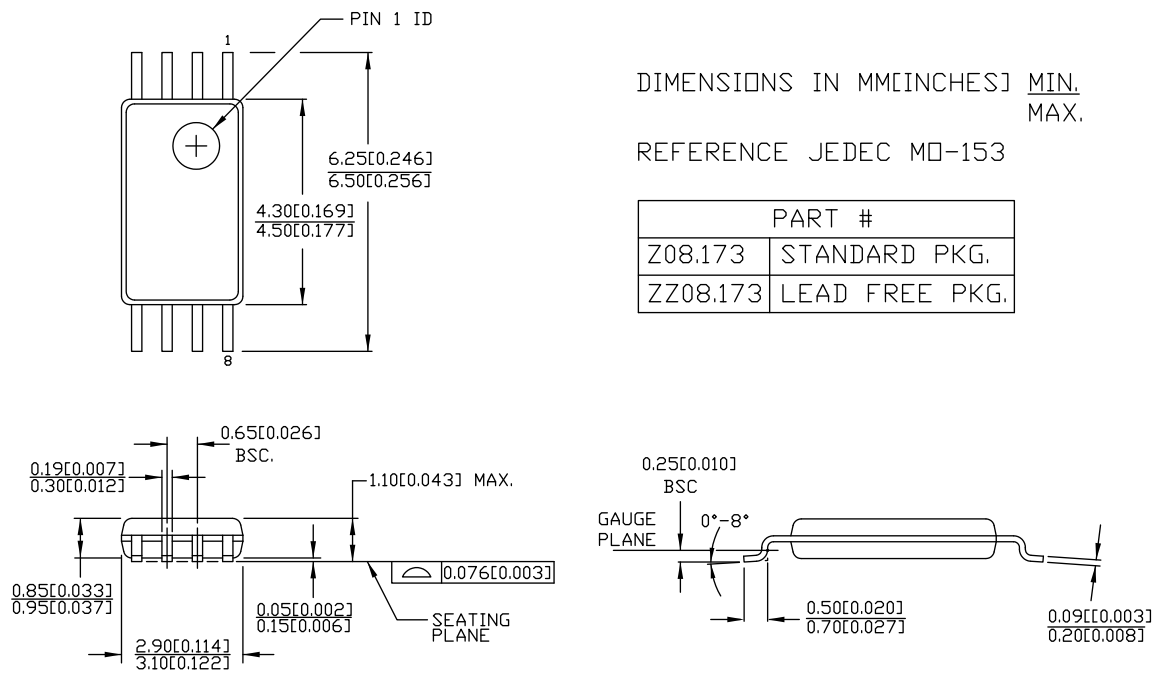
Figure 7. 8-pin TSSOP (4.40 mm Body) Z08.173/ZZ08.173 Package Outline, 51-85093
