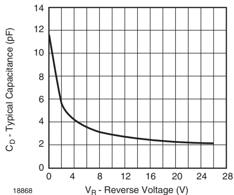
Fig. 2 - Typical Capacitance vs. Reverse Applied Voltage
