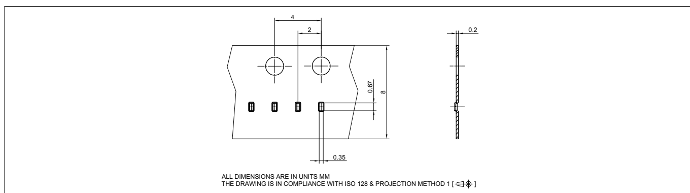
Figure 14 WLL-2-3 packing
