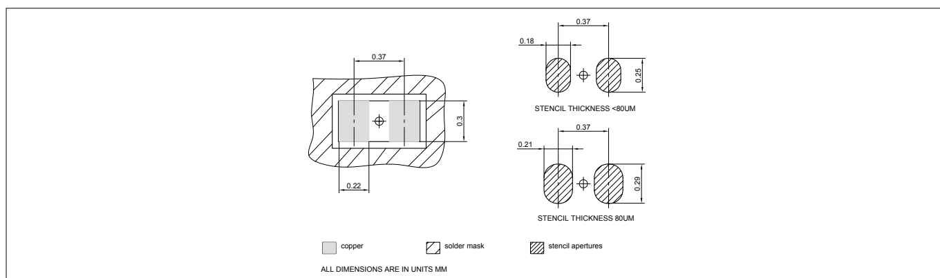
Figure 13 WLL-2-3 footprint ( recommendation for printed circuit board assembly see [2] )
