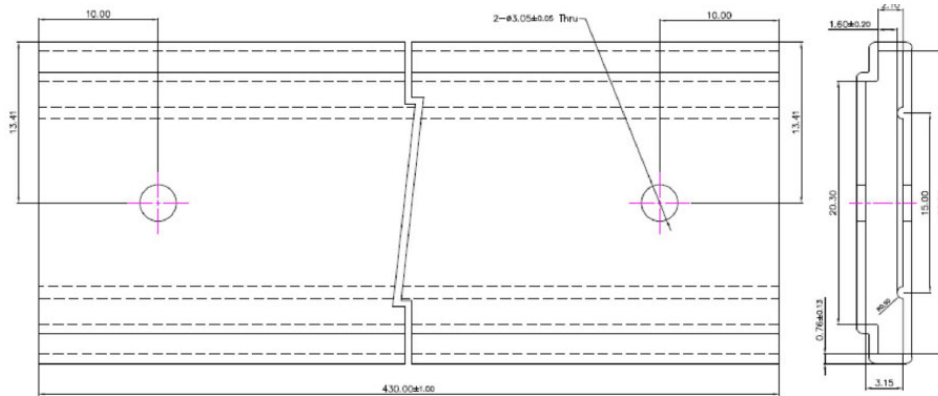
Figure 9c. Tube dimensions for L2C5-xxxx120xx1300 and L2C5-xxxx1208x1500.
