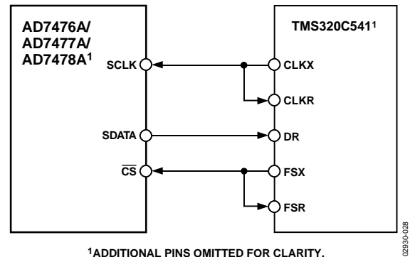
Figure 28. Interfacing to the TMS320C541
